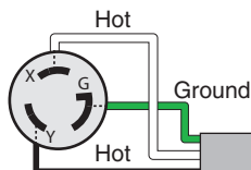
L6-30 PLUG (AS RECOMMENDED)
